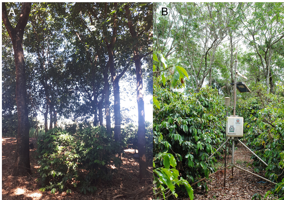
Figure 1 – (A) Double alleys of rubber trees intercropped with coffee trees. (B) Automatic weather station installed at the mean distance between the double alleys spaced 16 m apart. Source: the authors (2018).
